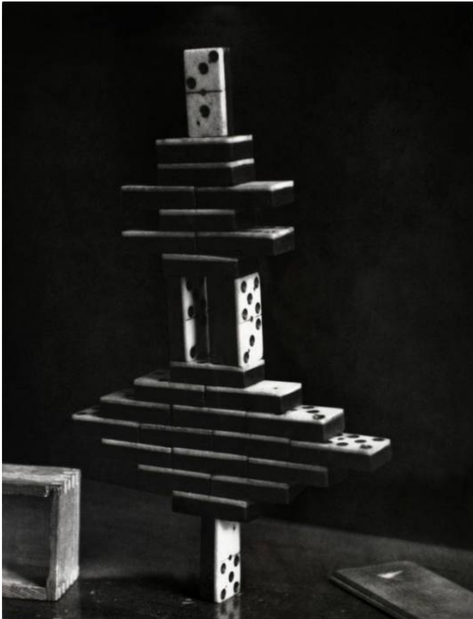
McDermott and McGough, Experiment upon the center of gravity made on a set of Dominoes
